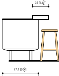
ELEVATION D
