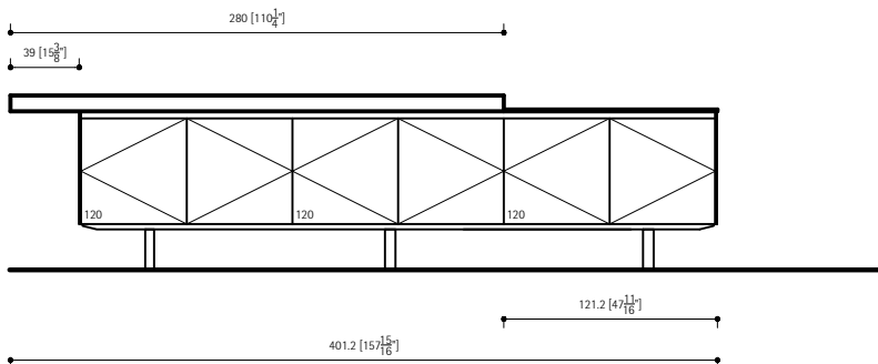
ELEVATION C
