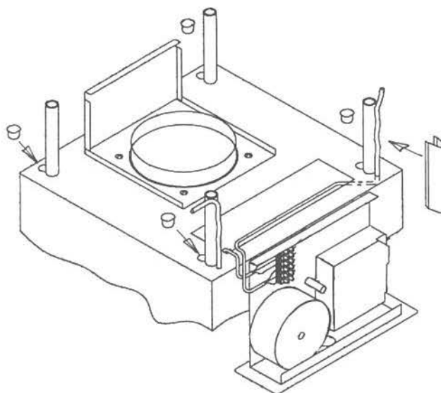
Turn duct 180°
